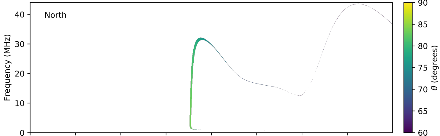
expres_earth_jupiter_io_jrm09_lossc-wid1deg_3kev_20140625_v01.cdf
