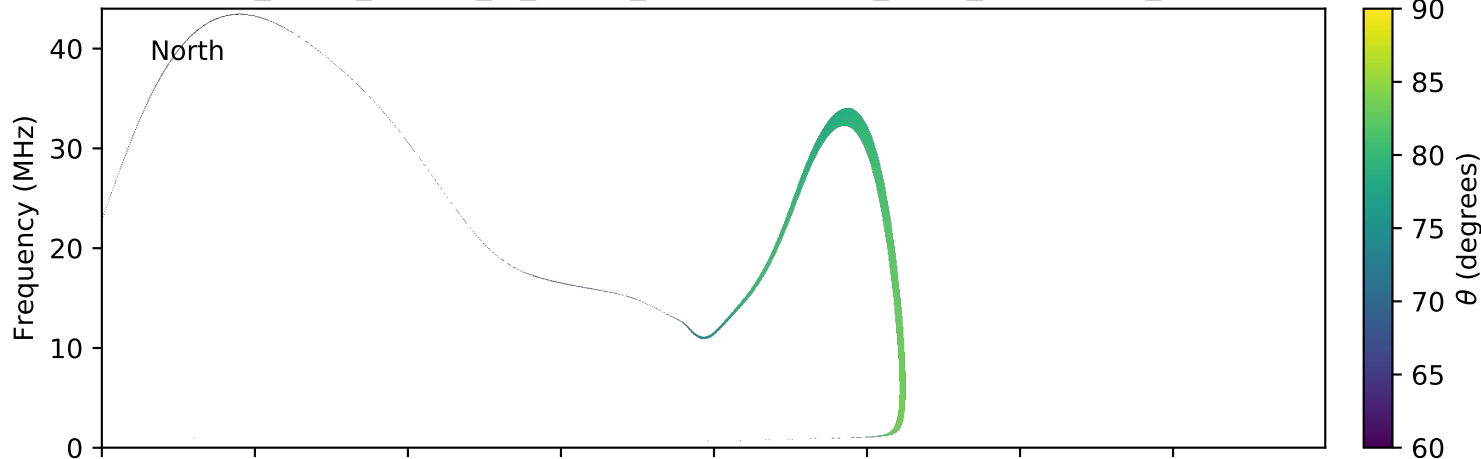
expres_earth_jupiter_io_jrm09_lossc-wid1deg_3kev_20140615_v01.cdf
