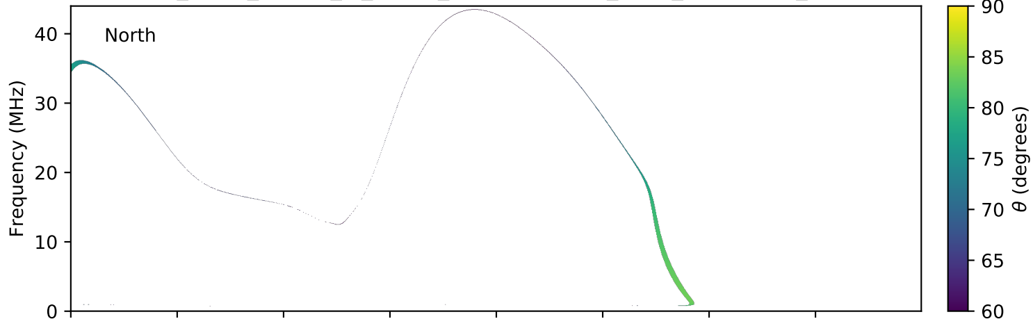
expres_earth_jupiter_io_jrm09_lossc-wid1deg_3kev_20140606_v01.cdf
