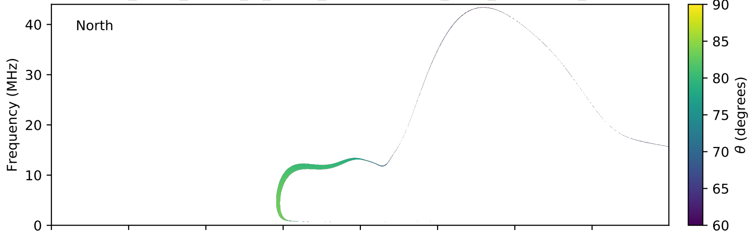
expres_earth_jupiter_io_jrm09_lossc-wid1deg_3kev_20140602_v01.cdf
