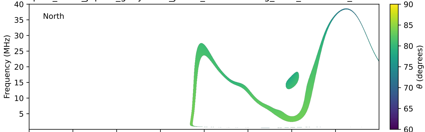
expres_earth_jupiter_ganymede_jrm33_lossc-wid1deg_3kev_20140620_v11.cdf
