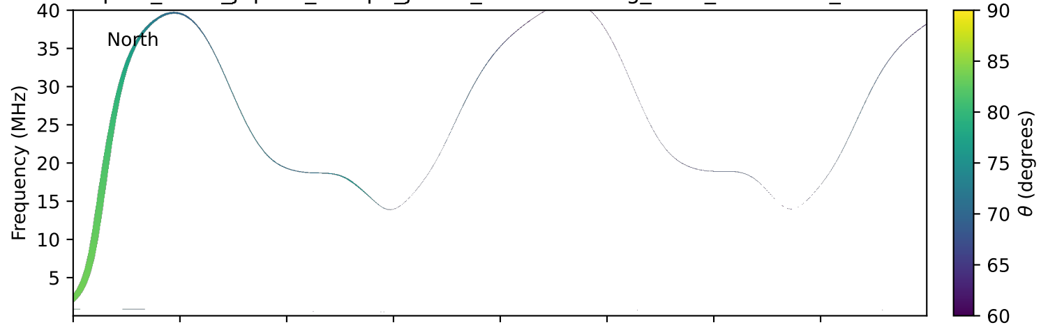
expres_earth_jupiter_europa_jrm33_lossc-wid1deg_3kev_20140603_v11.cdf
