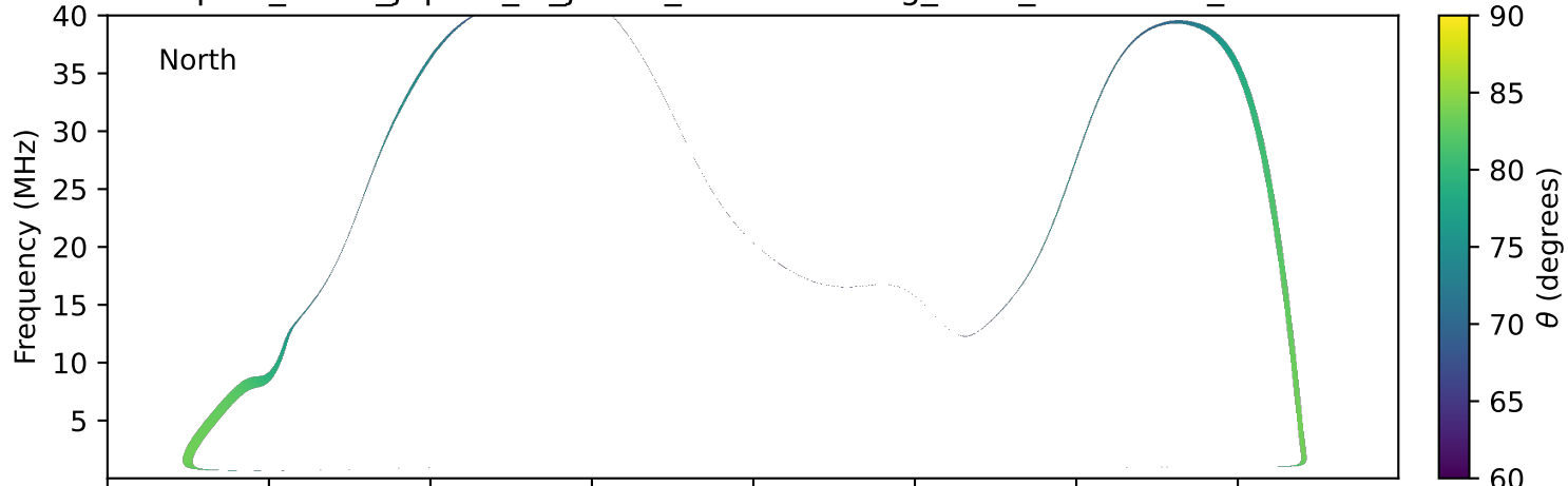
expres_earth_jupiter_io_jrm33_lossc-wid1deg_3kev_20140528_v11.cdf
