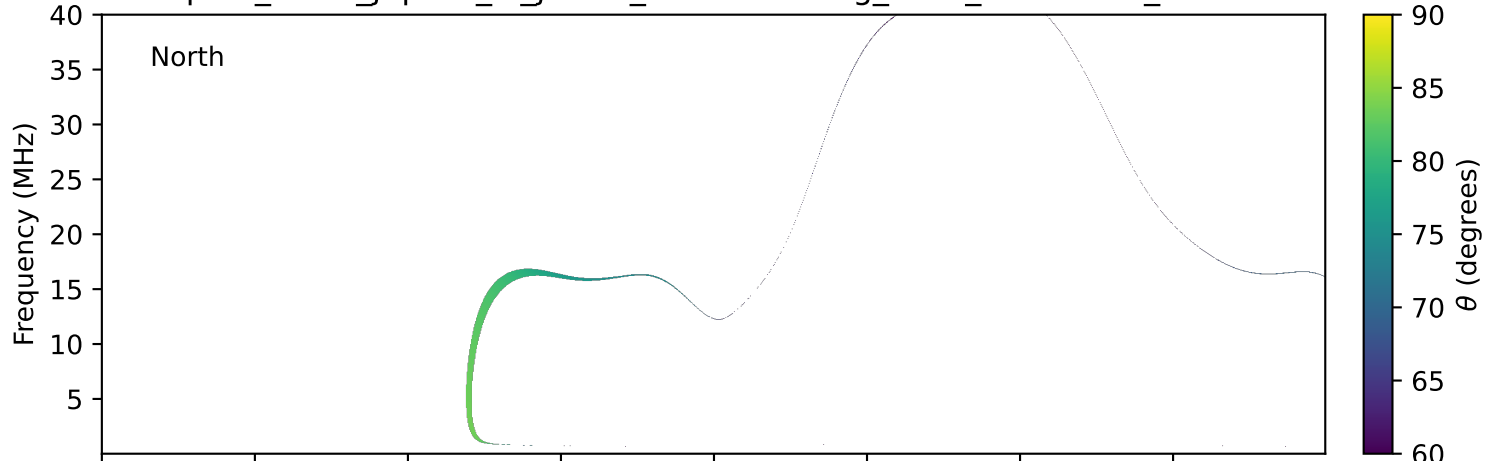
expres_earth_jupiter_io_jrm33_lossc-wid1deg_3kev_20140526_v11.cdf
