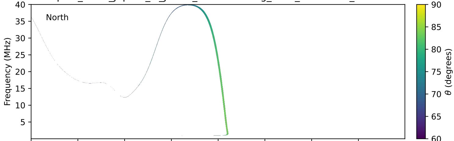
expres_earth_jupiter_io_jrm33_lossc-wid1deg_3kev_20140516_v11.cdf
