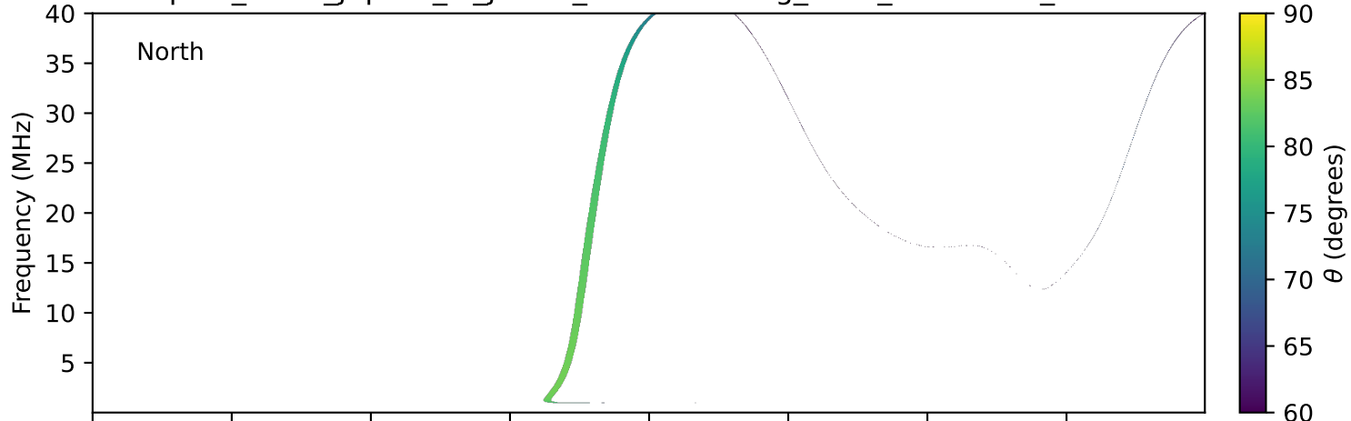
expres_earth_jupiter_io_jrm33_lossc-wid1deg_3kev_20140510_v11.cdf
