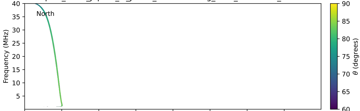
expres_earth_jupiter_io_jrm33_lossc-wid1deg_3kev_20140504_v11.cdf
