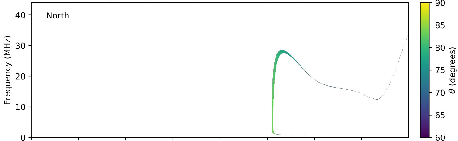
expres_earth_jupiter_io_jrm09_lossc-wid1deg_3kev_20140531_v01.cdf
