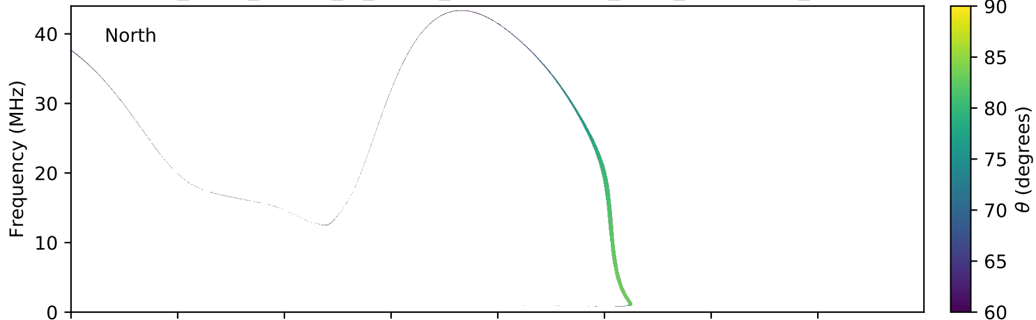
expres_earth_jupiter_io_jrm09_lossc-wid1deg_3kev_20140530_v01.cdf
