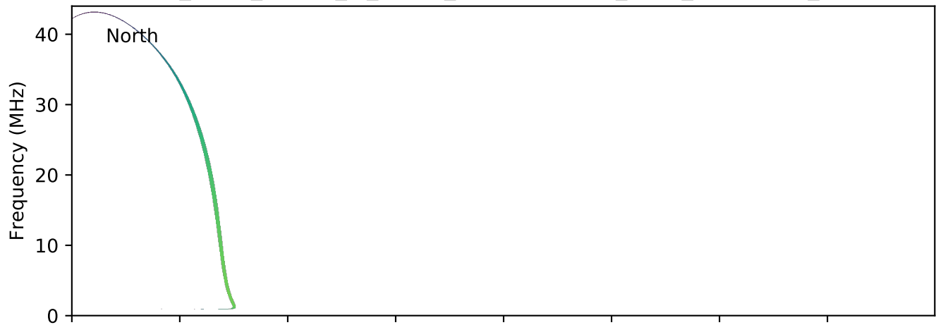
expres_earth_jupiter_io_jrm09_lossc-wid1deg_3kev_20140511_v01.cdf
