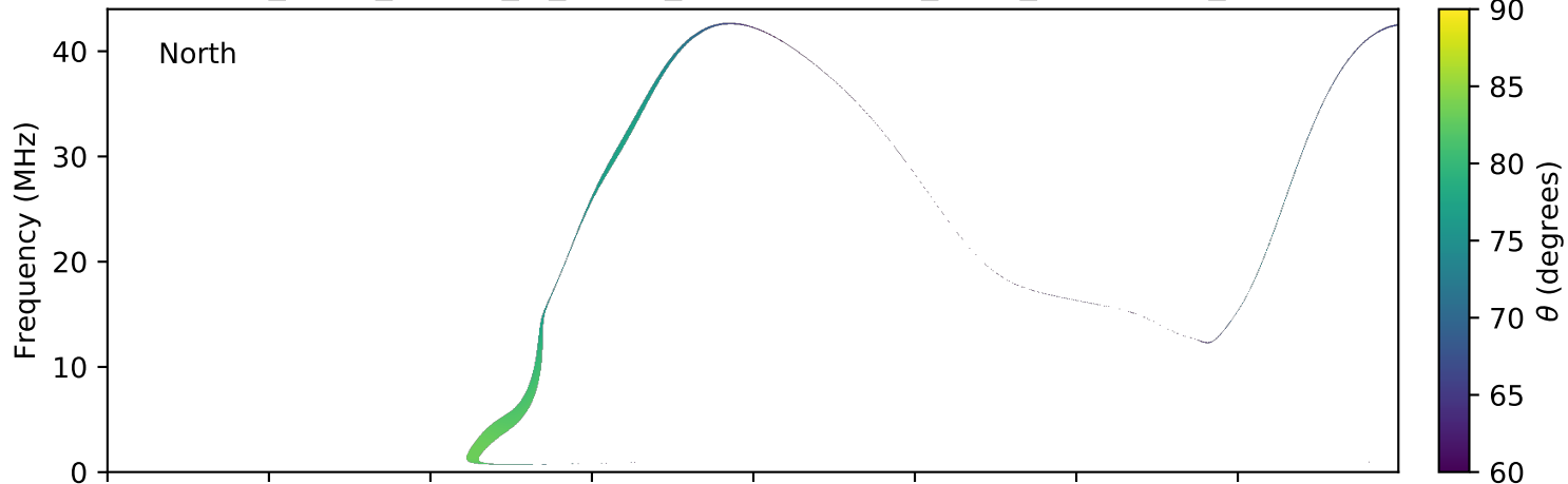
expres_earth_jupiter_io_jrm09_lossc-wid1deg_3kev_20140503_v01.cdf
