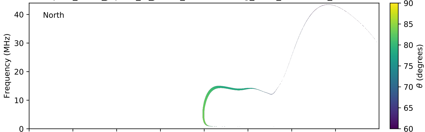
expres_earth_jupiter_io_jrm09_lossc-wid1deg_3kev_20140501_v01.cdf
