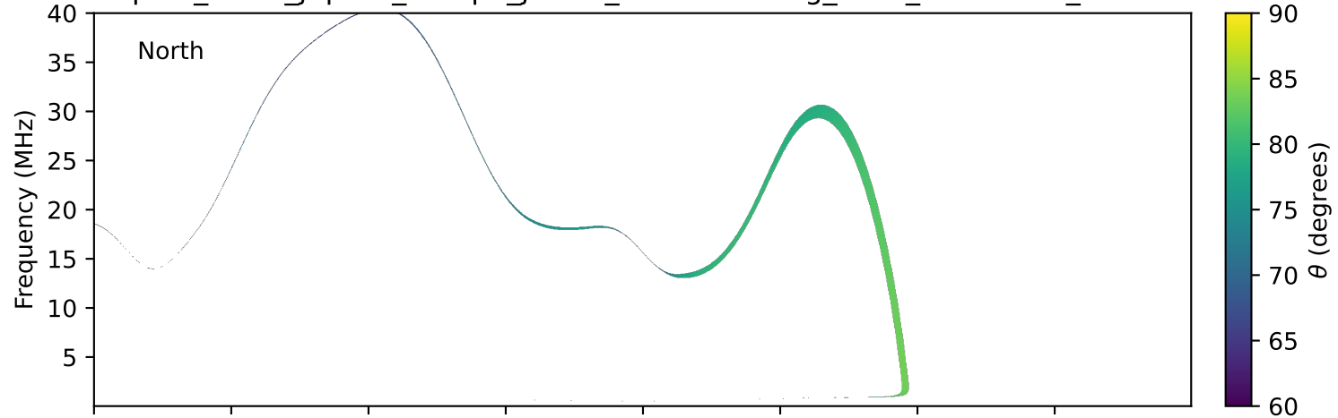
expres_earth_jupiter_europa_jrm33_lossc-wid1deg_3kev_20140517_v11.cdf
