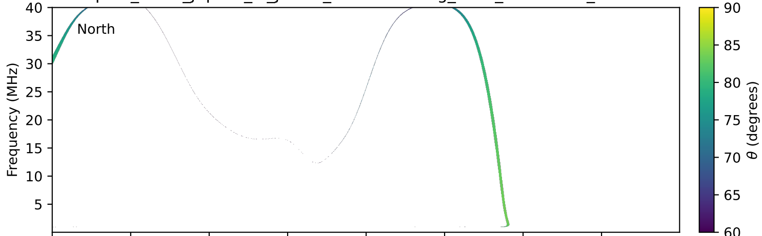
expres_earth_jupiter_io_jrm33_lossc-wid1deg_3kev_20140421_v11.cdf
