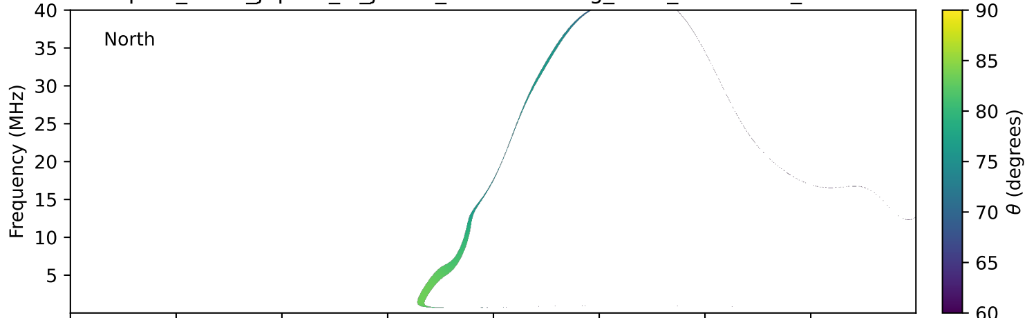
expres_earth_jupiter_io_jrm33_lossc-wid1deg_3kev_20140401_v11.cdf
