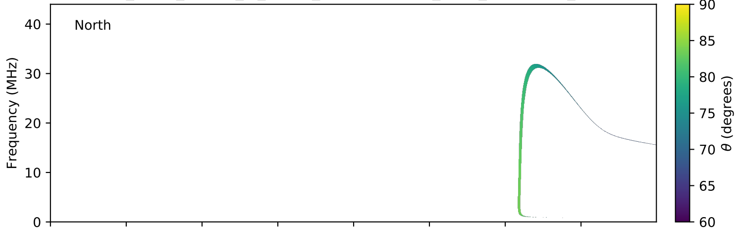
expres_earth_jupiter_io_jrm09_lossc-wid1deg_3kev_20140429_v01.cdf
