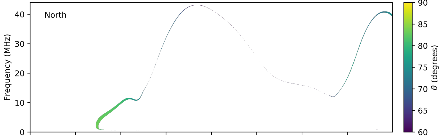
expres_earth_jupiter_io_jrm09_lossc-wid1deg_3kev_20140426_v01.cdf
