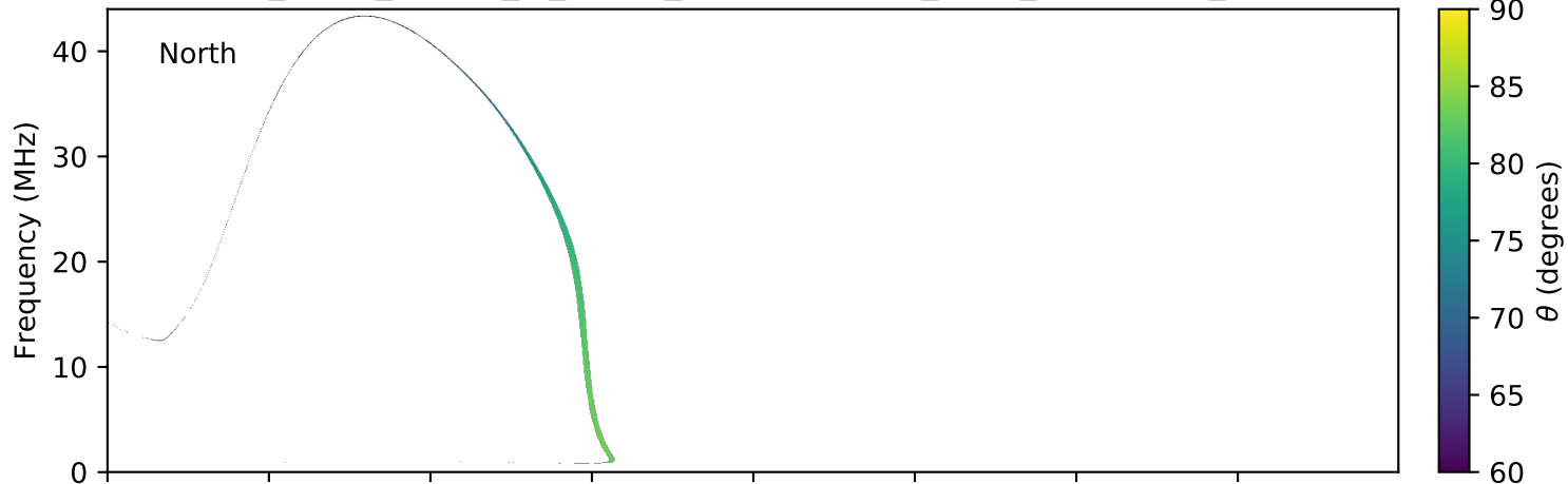
expres_earth_jupiter_io_jrm09_lossc-wid1deg_3kev_20140416_v01.cdf
