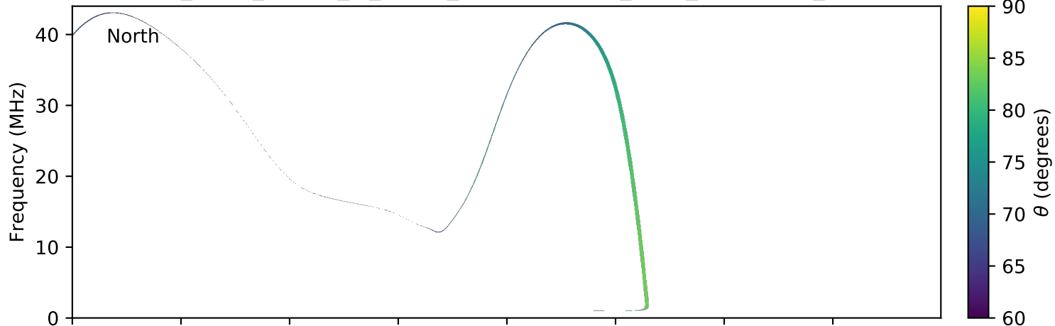
expres_earth_jupiter_io_jrm09_lossc-wid1deg_3kev_20140414_v01.cdf
