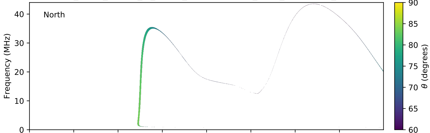
expres_earth_jupiter_io_jrm09_lossc-wid1deg_3kev_20140410_v01.cdf
