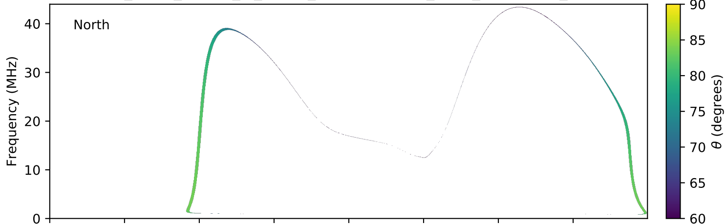
expres_earth_jupiter_io_jrm09_lossc-wid1deg_3kev_20140403_v01.cdf
