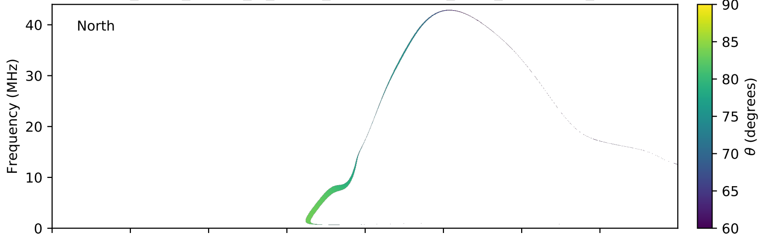
expres_earth_jupiter_io_jrm09_lossc-wid1deg_3kev_20140401_v01.cdf
