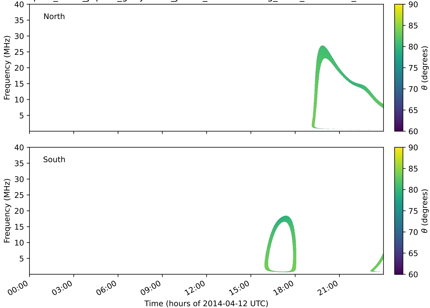
expres_earth_jupiter_ganymede_jrm33_lossc-wid1deg_3kev_20140412_v11.cdf
