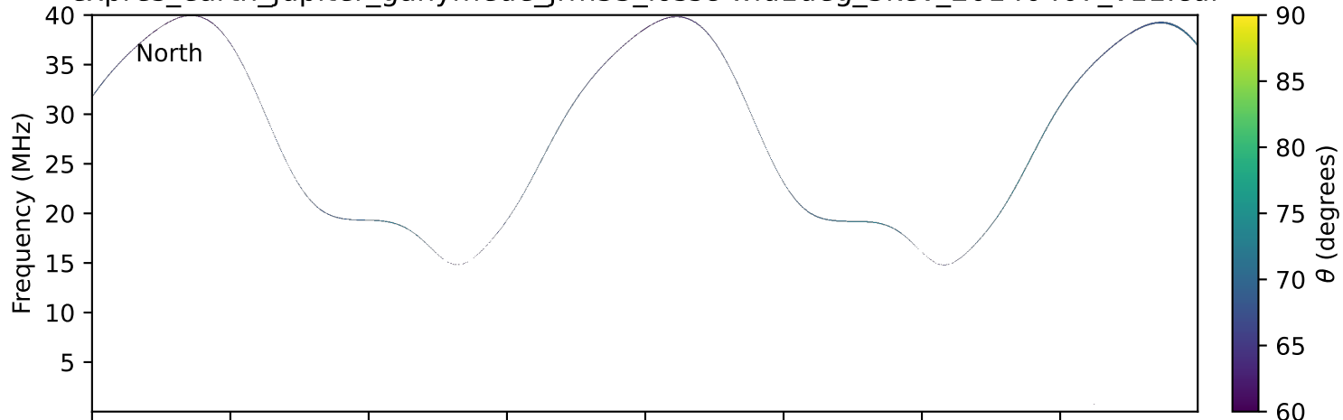
expres_earth_jupiter_ganymede_jrm33_lossc-wid1deg_3kev_20140407_v11.cdf
