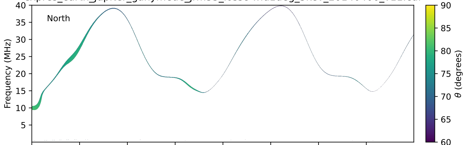
expres_earth_jupiter_ganymede_jrm33_lossc-wid1deg_3kev_20140406_v11.cdf
