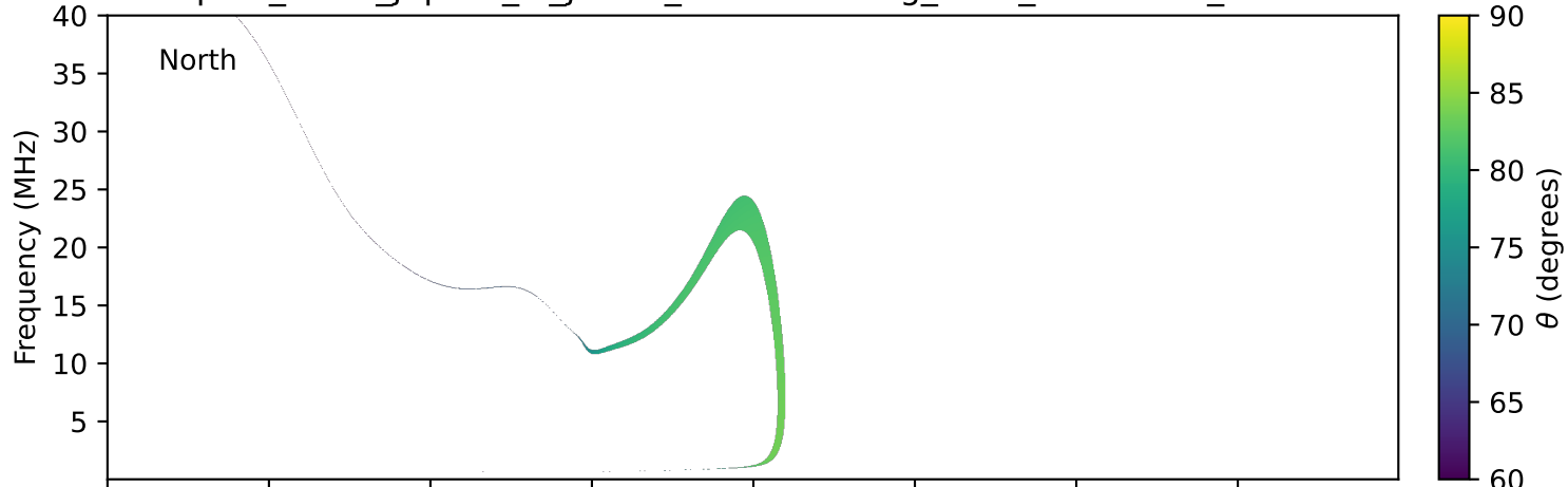
expres_earth_jupiter_io_jrm33_lossc-wid1deg_3kev_20140331_v11.cdf
