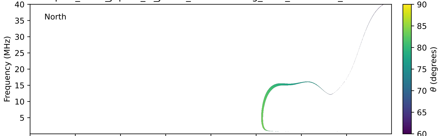
expres_earth_jupiter_io_jrm33_lossc-wid1deg_3kev_20140330_v11.cdf
