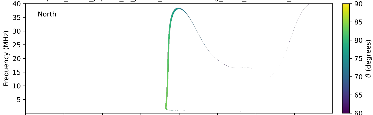
expres_earth_jupiter_io_jrm33_lossc-wid1deg_3kev_20140309_v11.cdf
