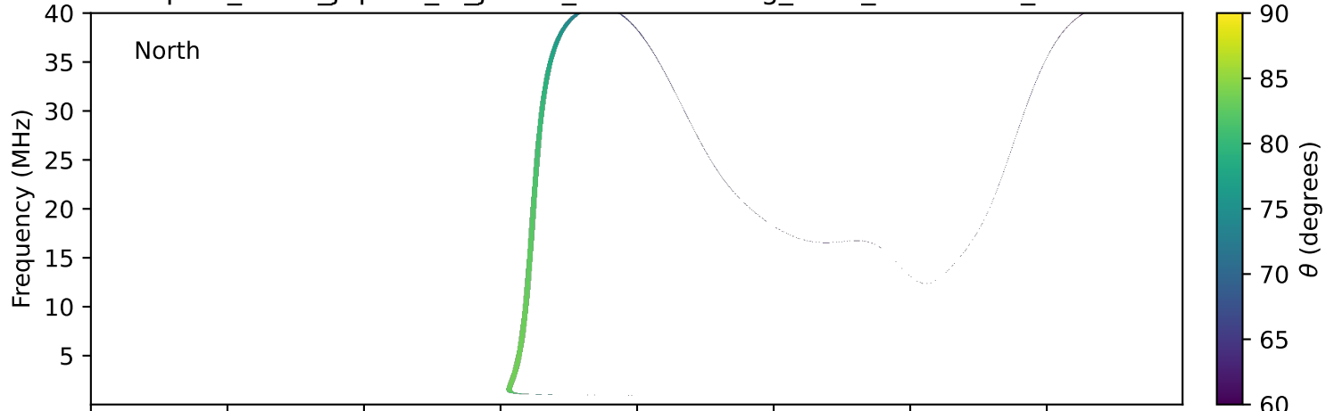
expres_earth_jupiter_io_jrm33_lossc-wid1deg_3kev_20140302_v11.cdf
