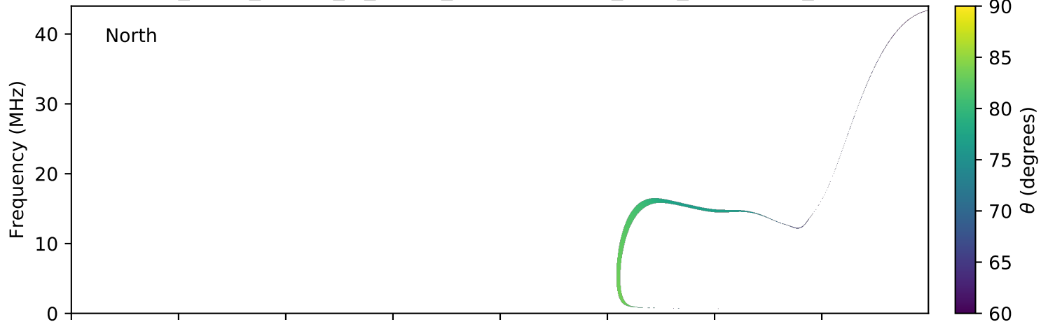
expres_earth_jupiter_io_jrm09_lossc-wid1deg_3kev_20140330_v01.cdf
