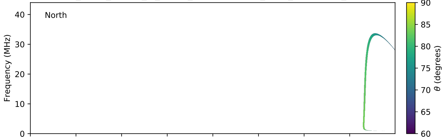
expres_earth_jupiter_io_jrm09_lossc-wid1deg_3kev_20140328_v01.cdf
