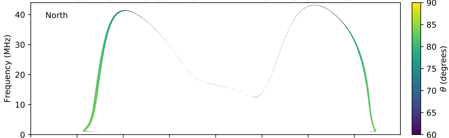
expres_earth_jupiter_io_jrm09_lossc-wid1deg_3kev_20140327_v01.cdf
