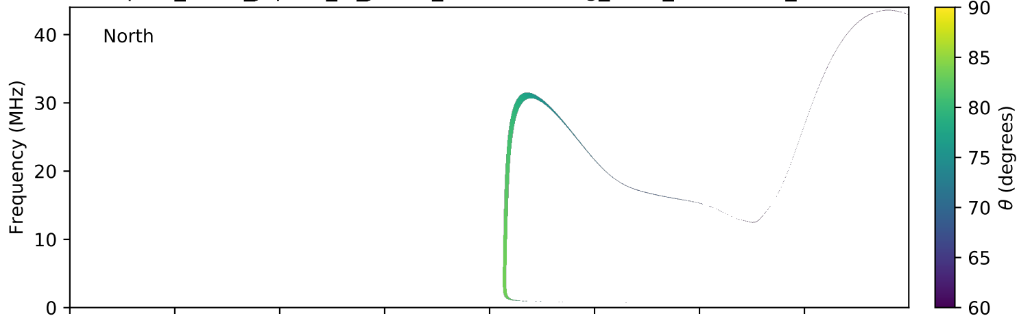
expres_earth_jupiter_io_jrm09_lossc-wid1deg_3kev_20140316_v01.cdf
