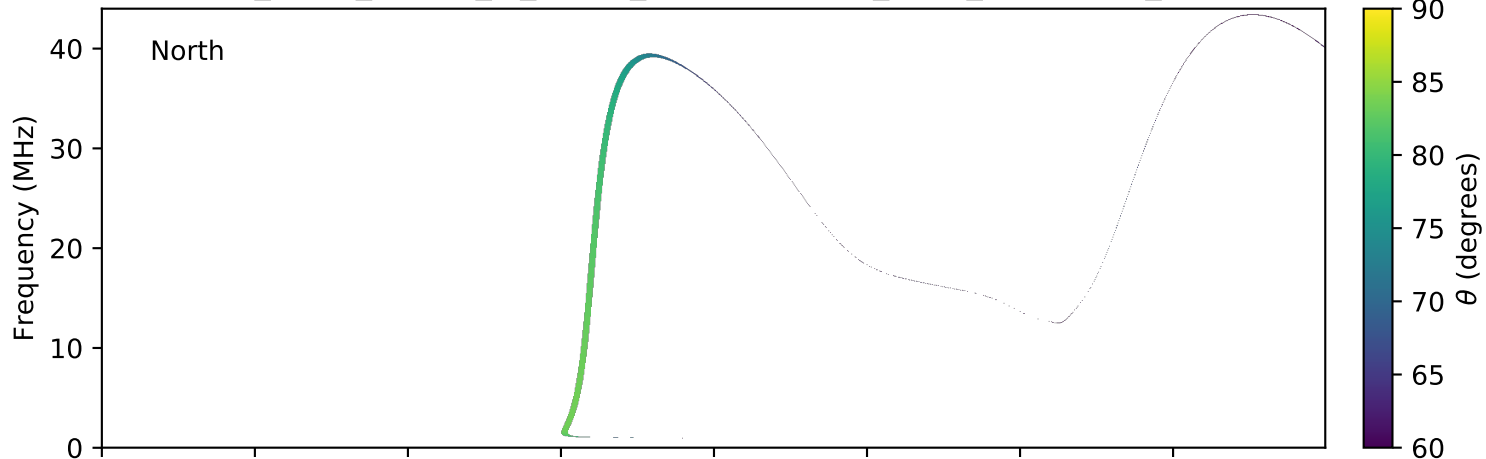
expres_earth_jupiter_io_jrm09_lossc-wid1deg_3kev_20140302_v01.cdf
