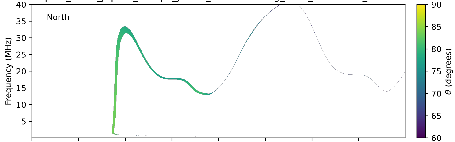
expres_earth_jupiter_europa_jrm33_lossc-wid1deg_3kev_20140320_v11.cdf
