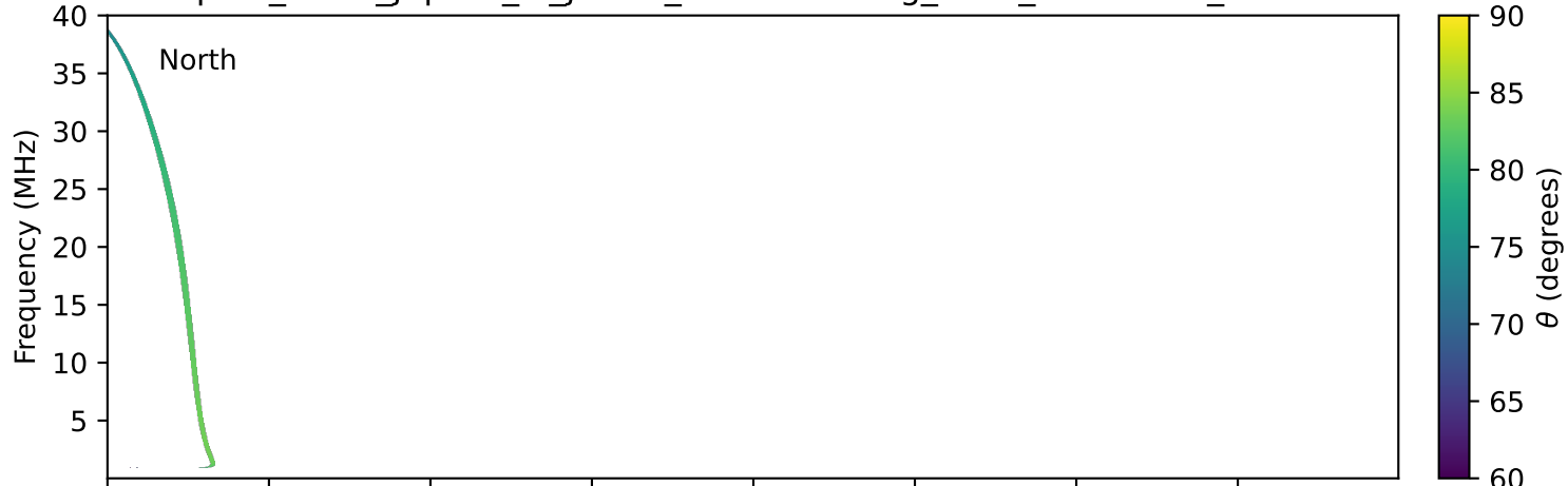
expres_earth_jupiter_io_jrm33_lossc-wid1deg_3kev_20140224_v11.cdf
