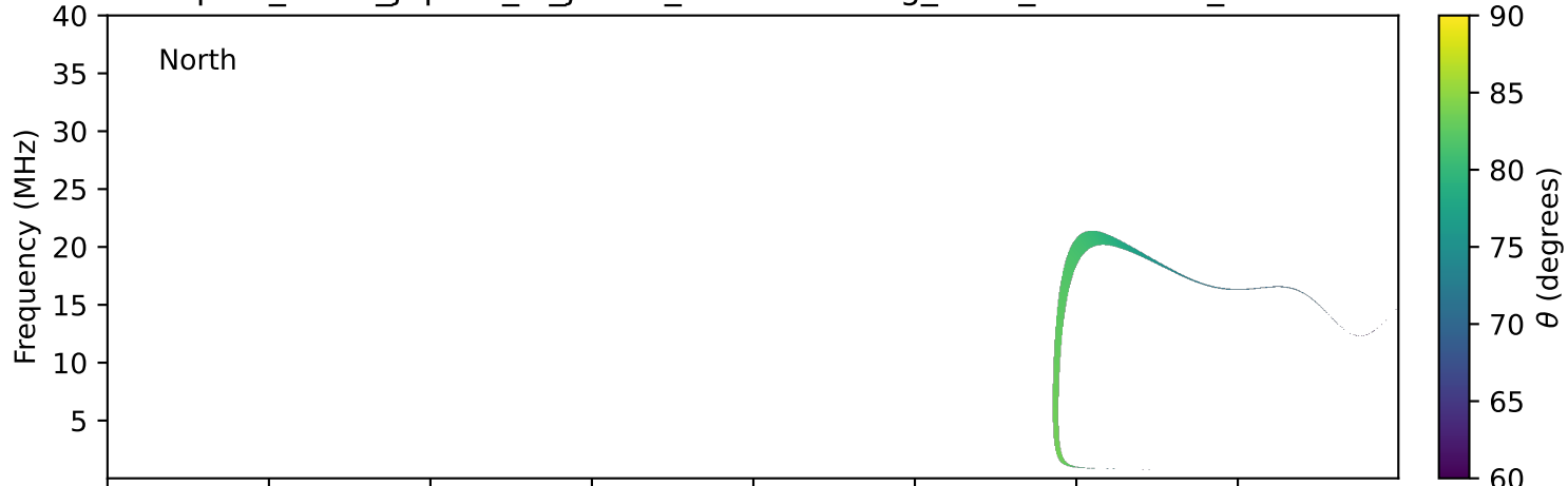
expres_earth_jupiter_io_jrm33_lossc-wid1deg_3kev_20140219_v11.cdf
