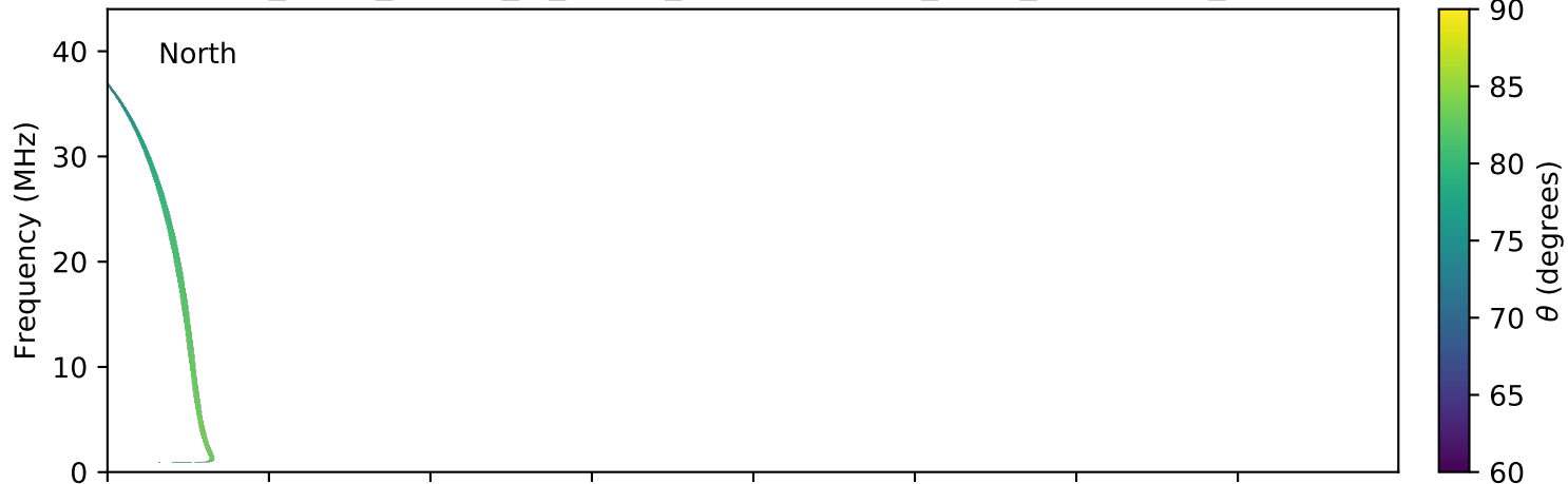
expres_earth_jupiter_io_jrm09_lossc-wid1deg_3kev_20140224_v01.cdf
