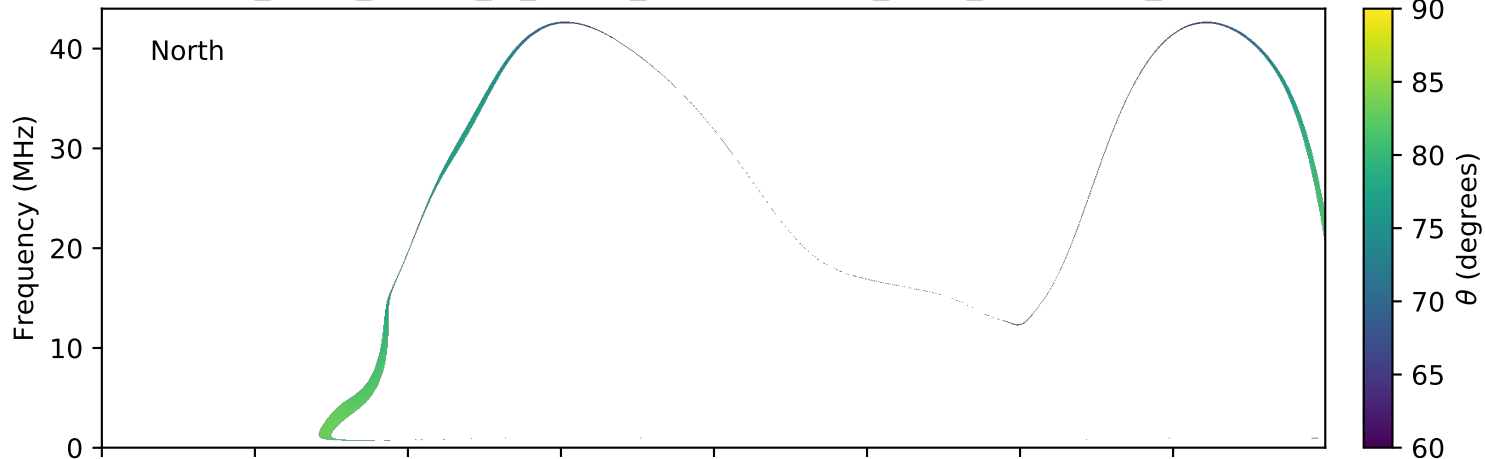
expres_earth_jupiter_io_jrm09_lossc-wid1deg_3kev_20140216_v01.cdf
