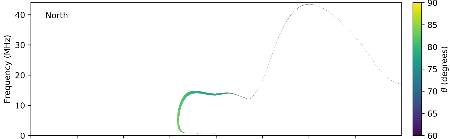
expres_earth_jupiter_io_jrm09_lossc-wid1deg_3kev_20140214_v01.cdf
