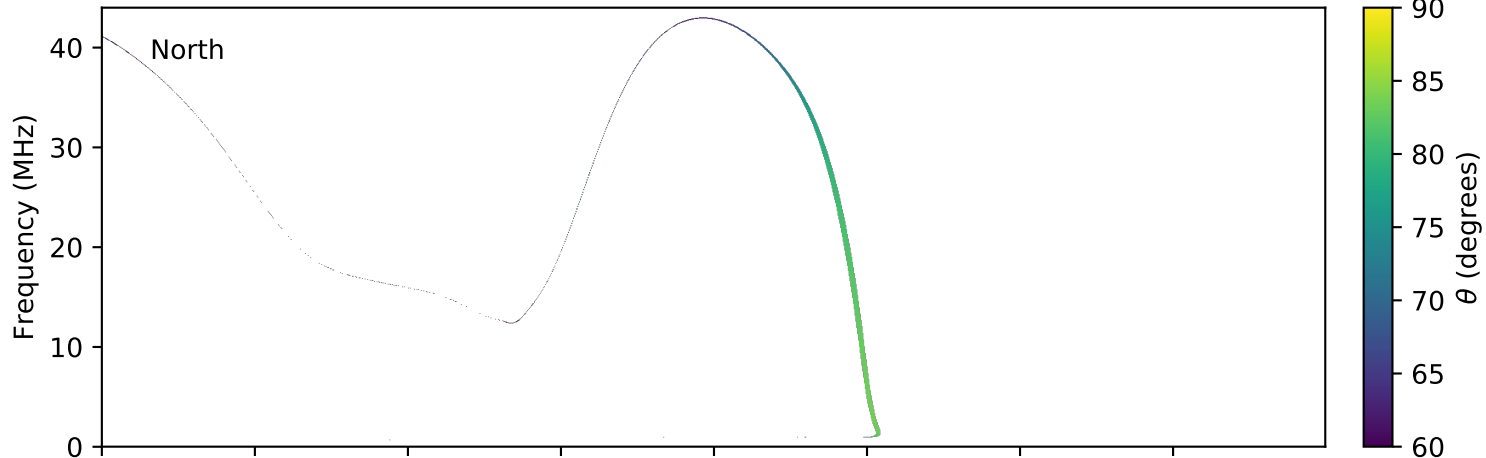
expres_earth_jupiter_io_jrm09_lossc-wid1deg_3kev_20140204_v01.cdf
