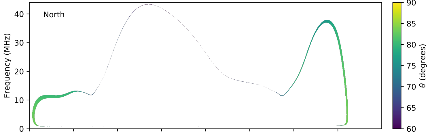
expres_earth_jupiter_io_jrm09_lossc-wid1deg_3kev_20140202_v01.cdf
