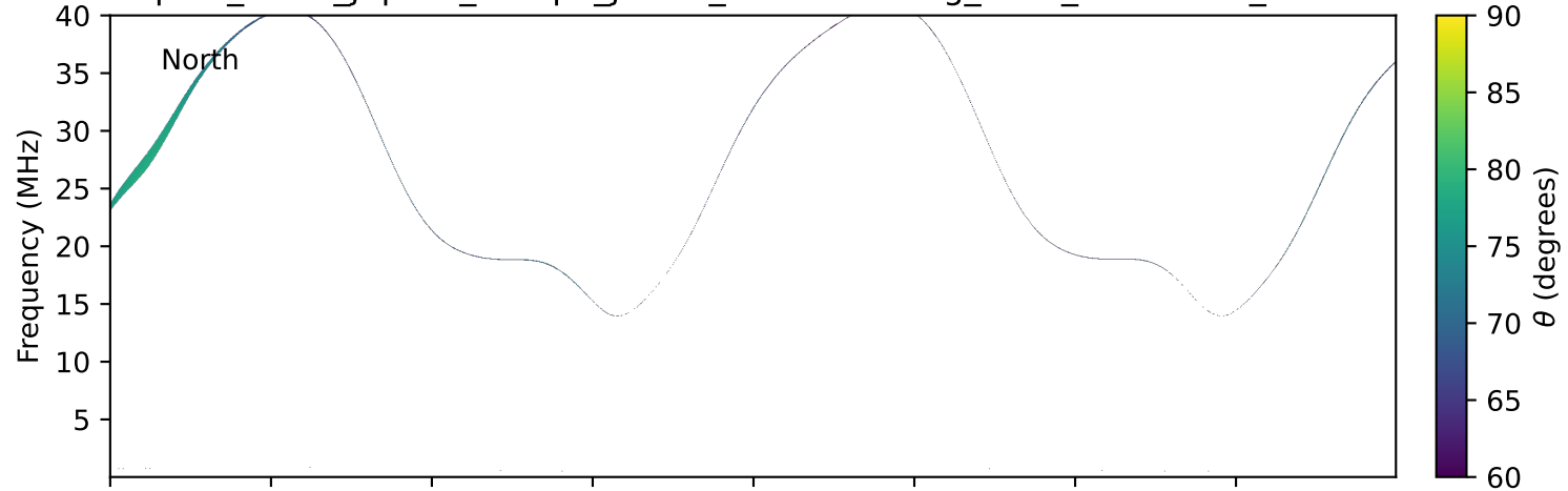
expres_earth_jupiter_europa_jrm33_lossc-wid1deg_3kev_20140220_v11.cdf
