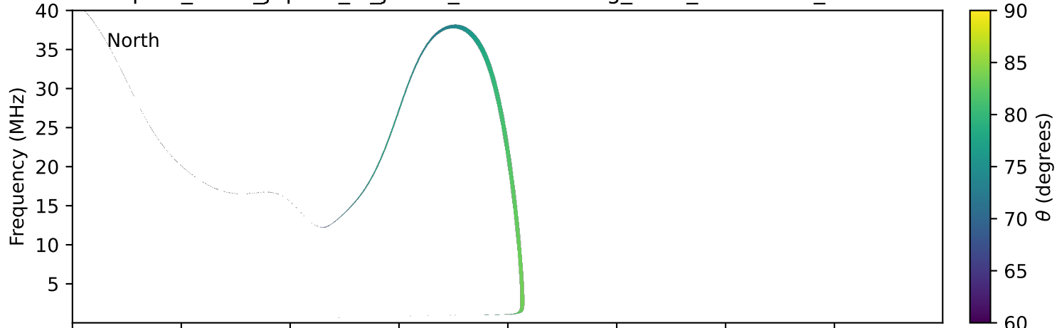
expres_earth_jupiter_io_jrm33_lossc-wid1deg_3kev_20140121_v11.cdf
