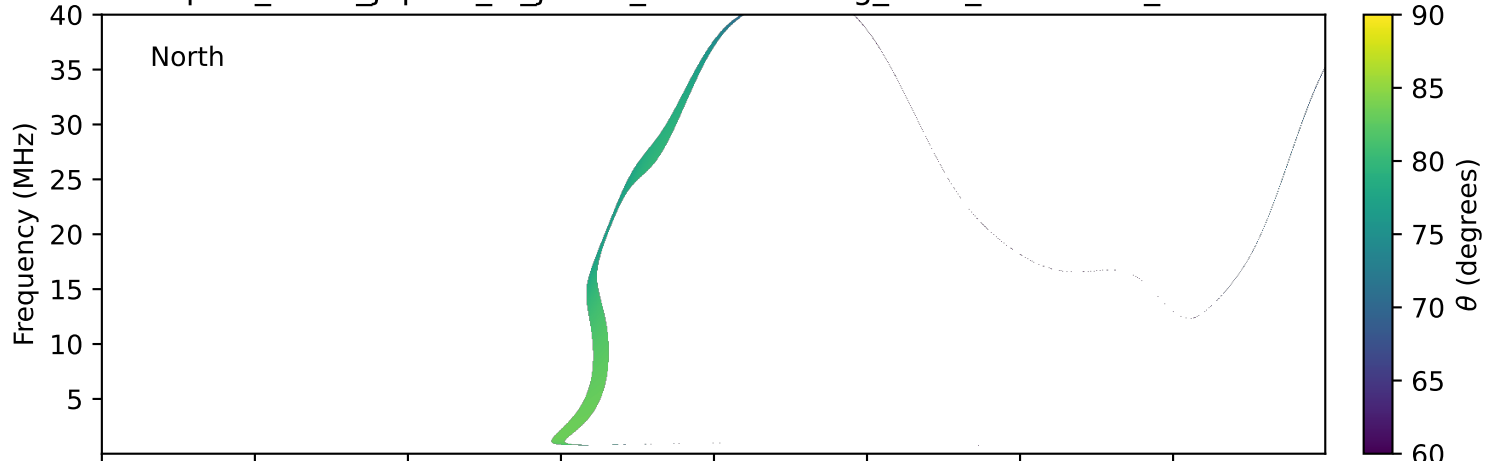
expres_earth_jupiter_io_jrm33_lossc-wid1deg_3kev_20140115_v11.cdf
