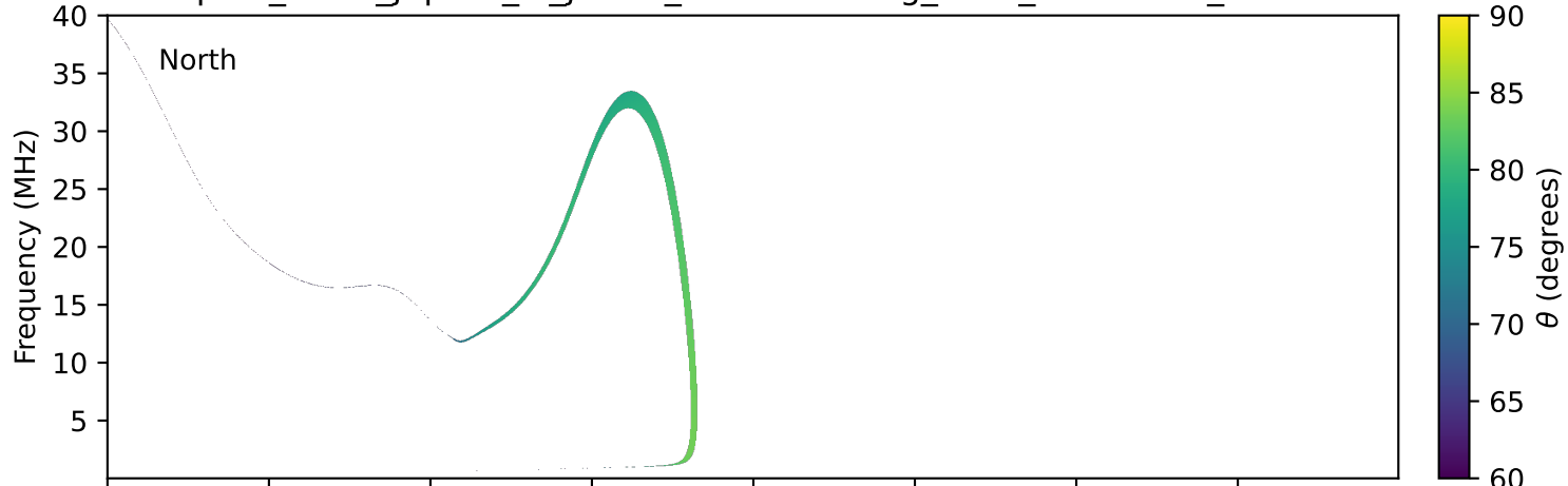
expres_earth_jupiter_io_jrm33_lossc-wid1deg_3kev_20140114_v11.cdf
